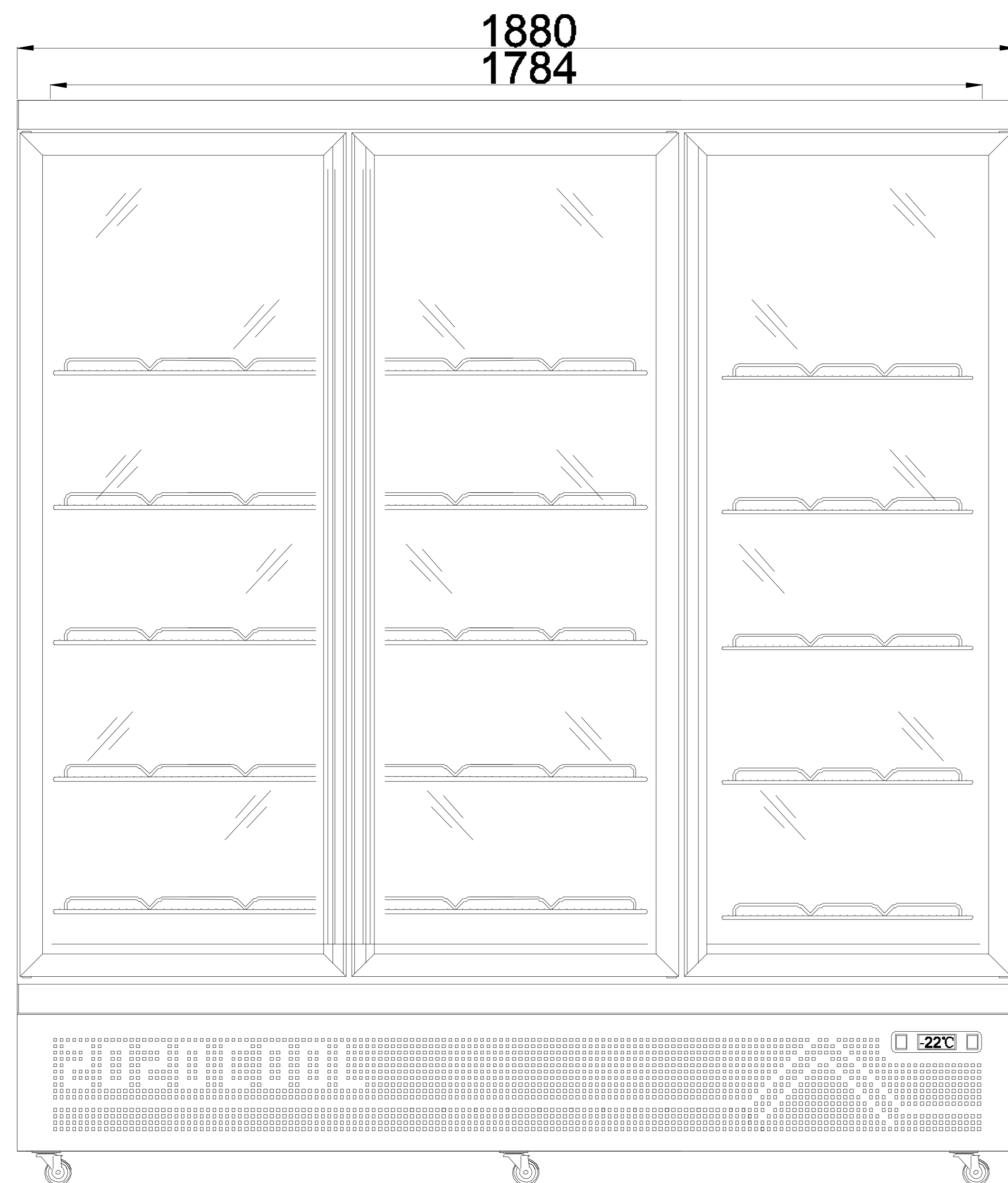
AISLEPRO Three Door Fridge (AISLEPRO 3D)
